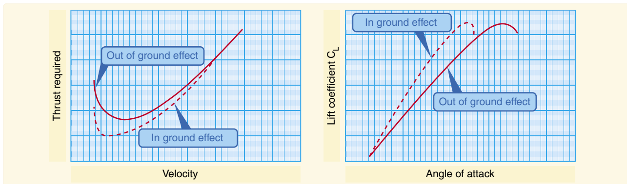
Figure 4-14. Ground effect changes drag and lift.
