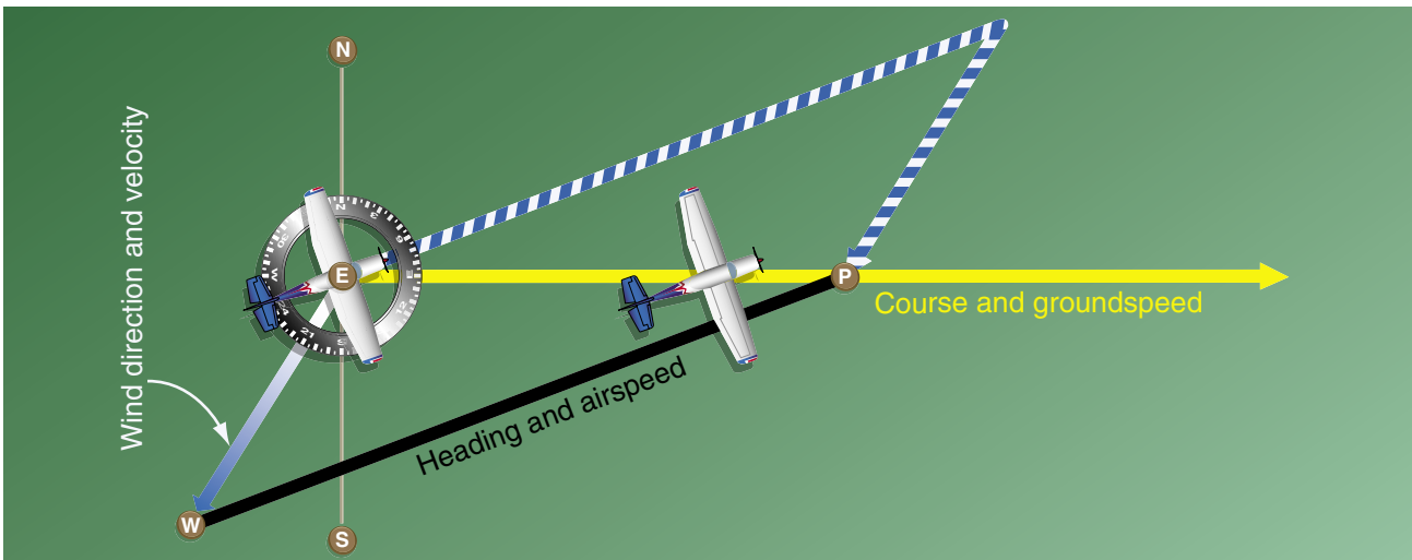
Figure 15-20. The wind triangle as is drawn in navigation practice.
