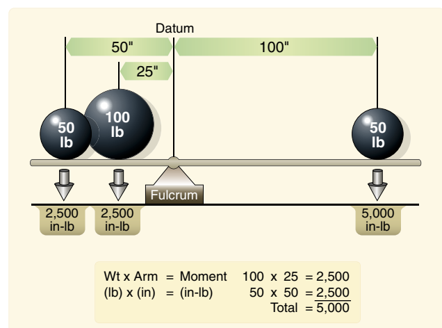
Figure 9-4. Establishing a balance.
