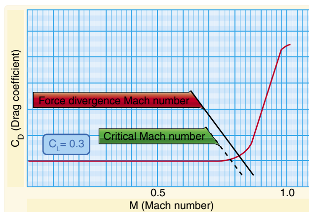
Figure 4-57. Critical Mach.
