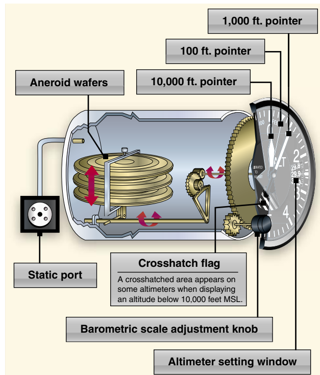
Figure 7-2. Altimeter.
