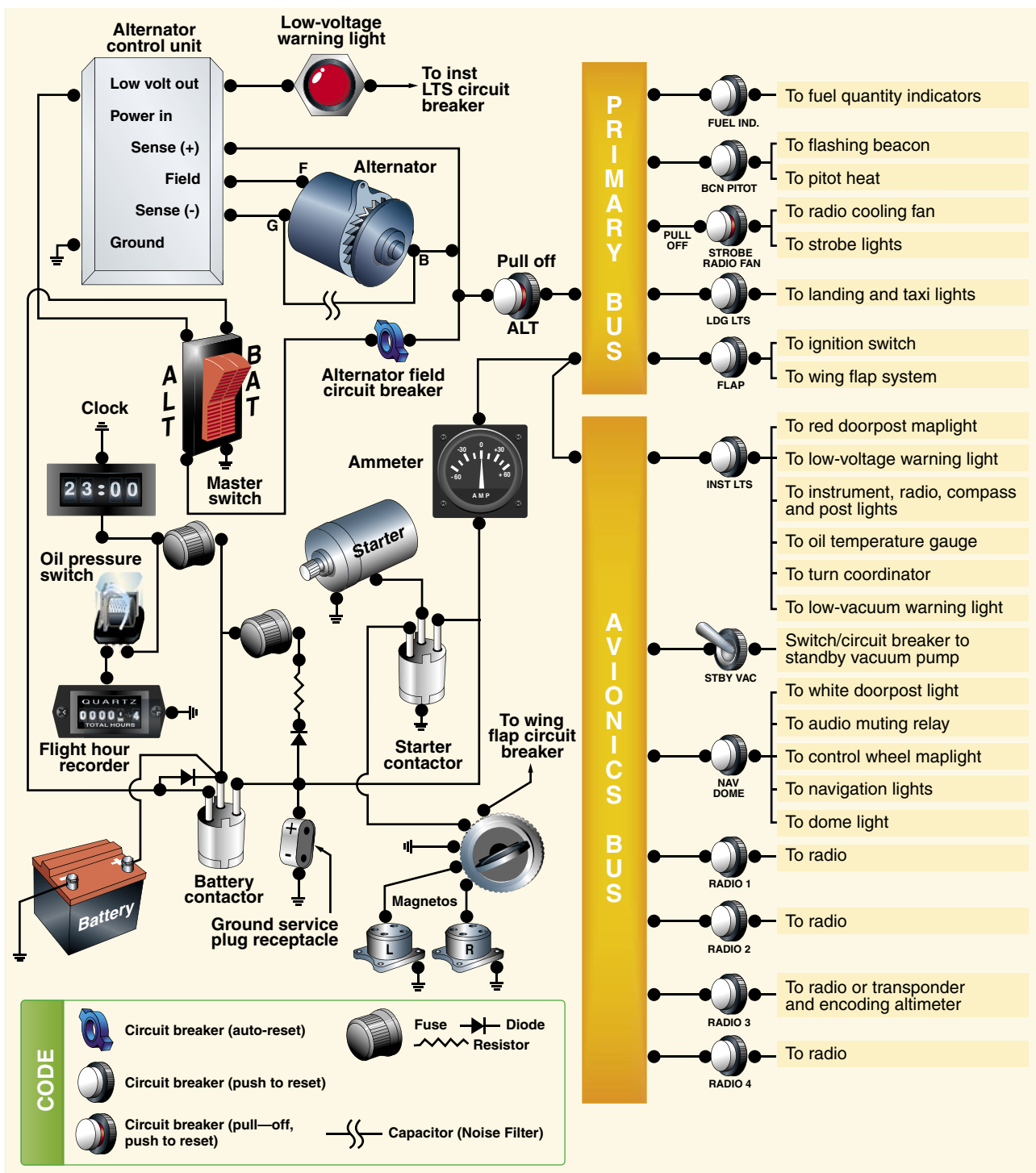
Figure 6-34. Electrical system schematic.
