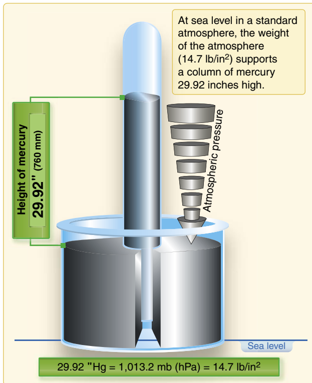
Figure 11-6. Mercurial barometer.
