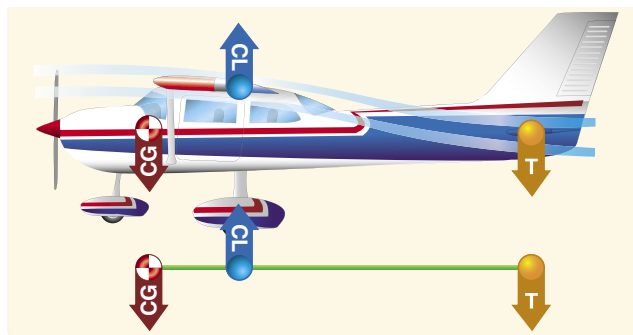
Figure 4-20. Longitudinal stability.
