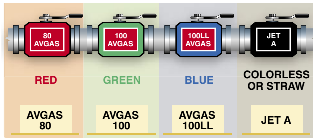
Figure 6-32. Aviation fuel color-coding system.
