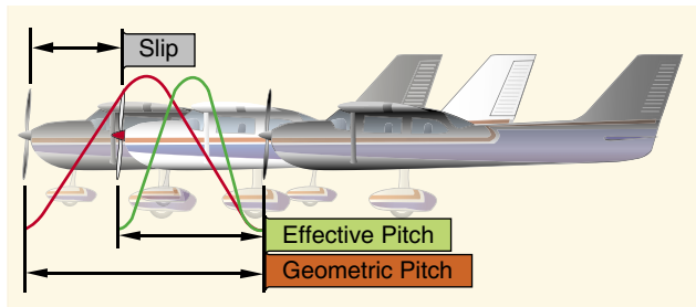
Figure 4-37. Propeller slippage.
