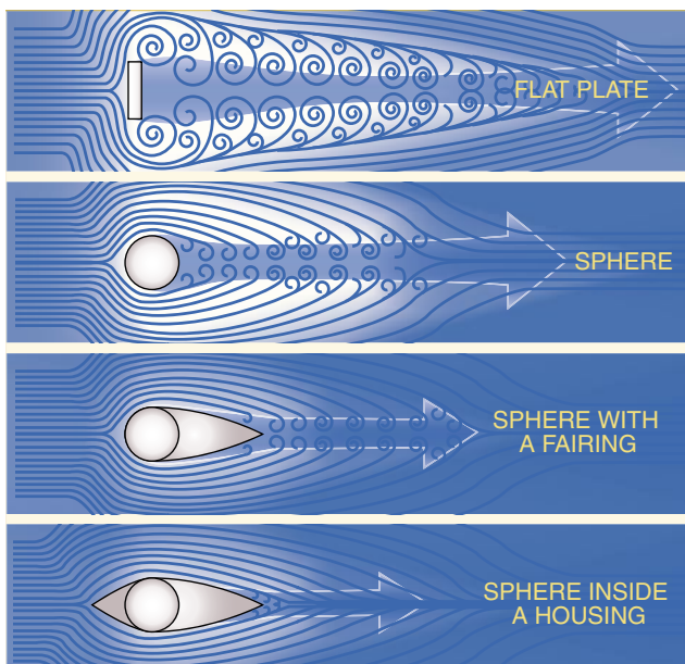
Figure 4-5. Form drag.
