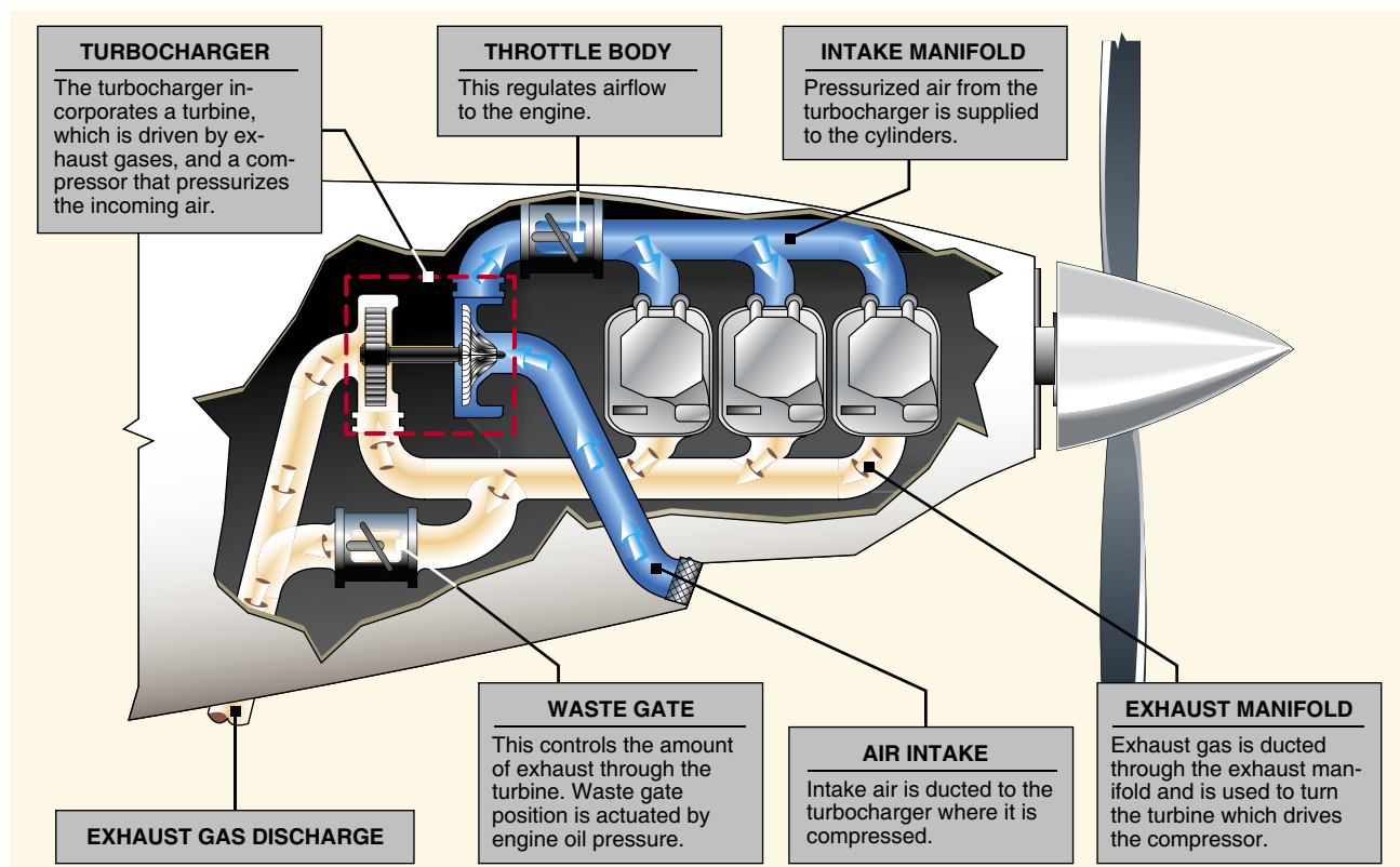
Figure 6-15. Turbocharger components.
