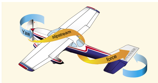
Figure 4-40. Corkscrewing slipstream.
