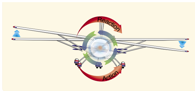
Figure 4-39. Torque reaction.
