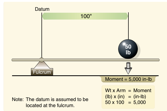
Figure 9-3. Determining moment.
