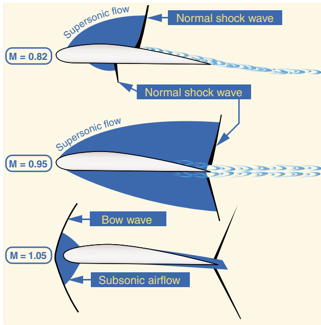
Figure 4-59. Shock waves.
