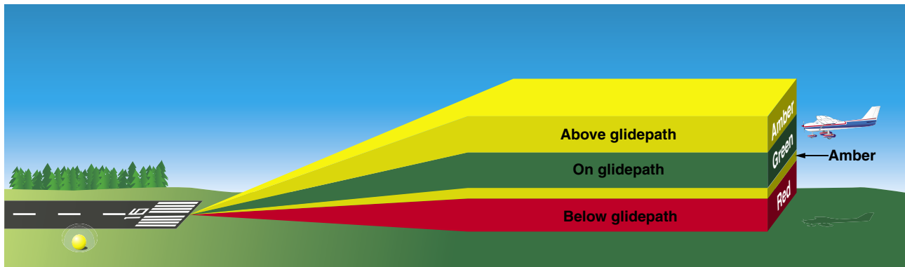
Figure 13-9. Tri-color visual approach slope indicator.
