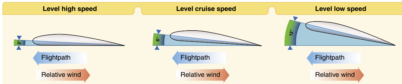
Figure 4-3. Angle of attack at various speeds.
