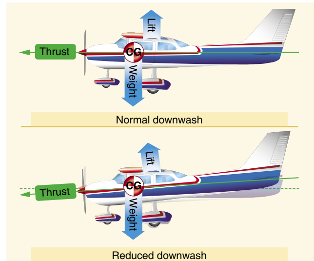
Figure 4-22. Reduced power allows pitch down.
